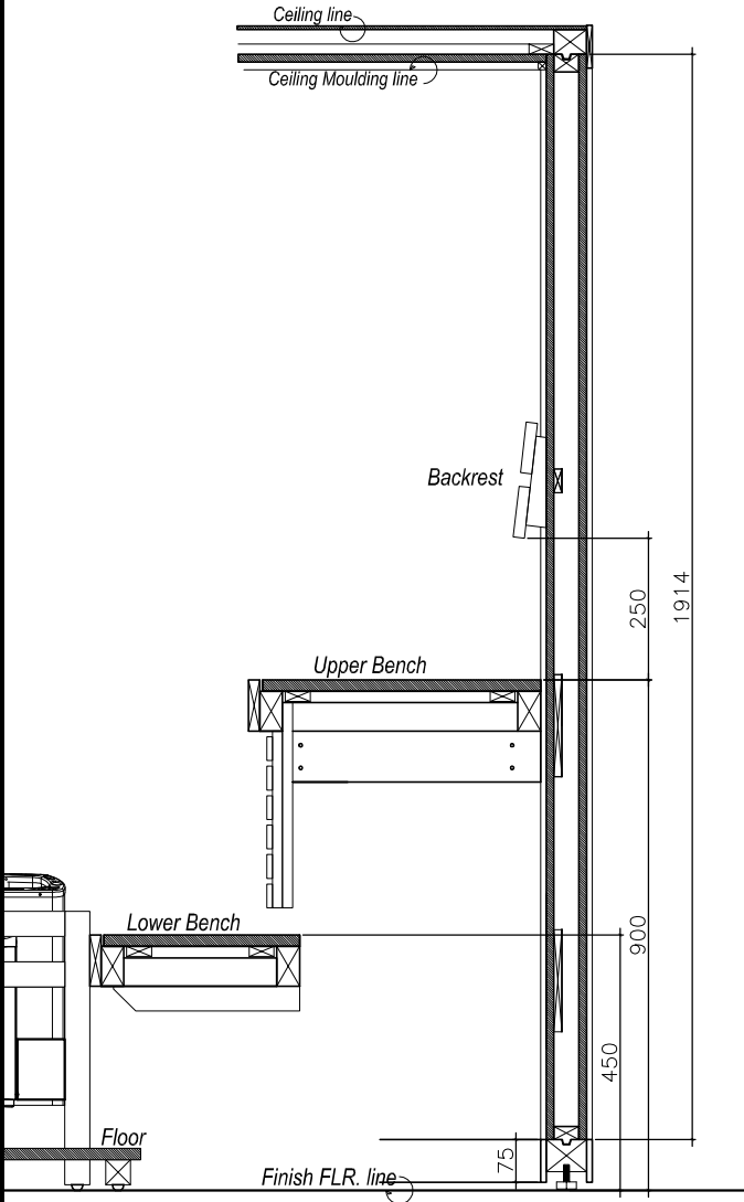
SECTION FIT TO SCALE
